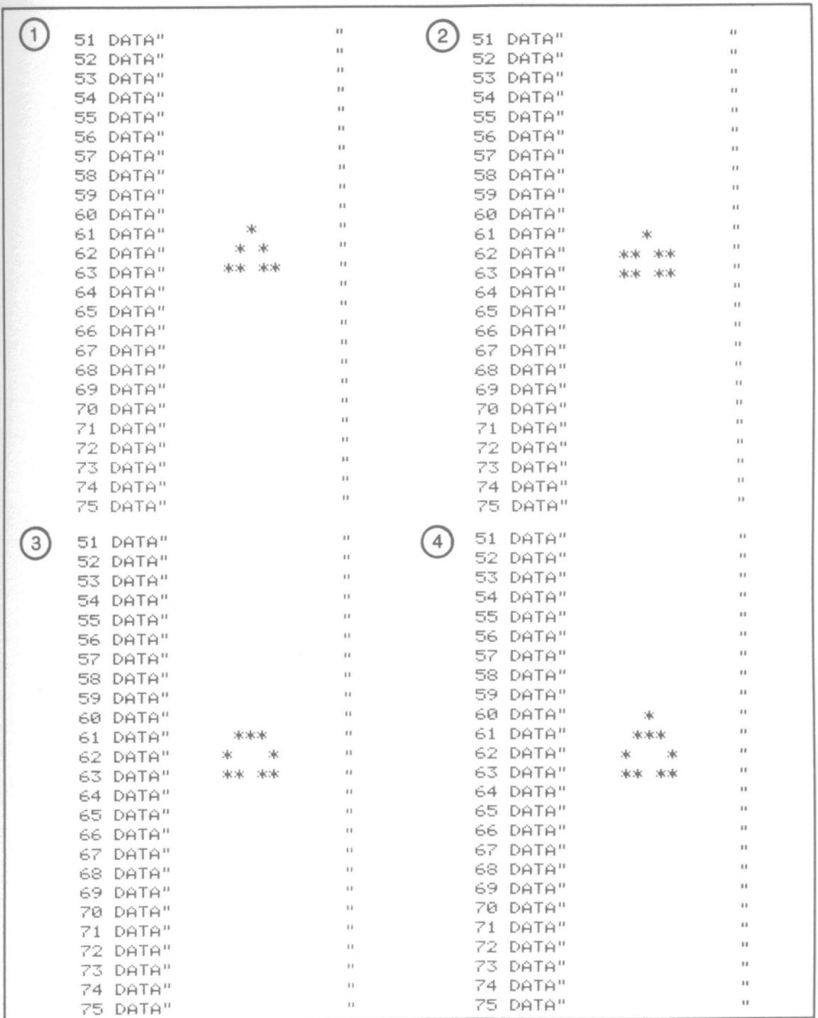
Fig. 2-3. The Data Statements in the Cellular Automaton program as they continue to change.
