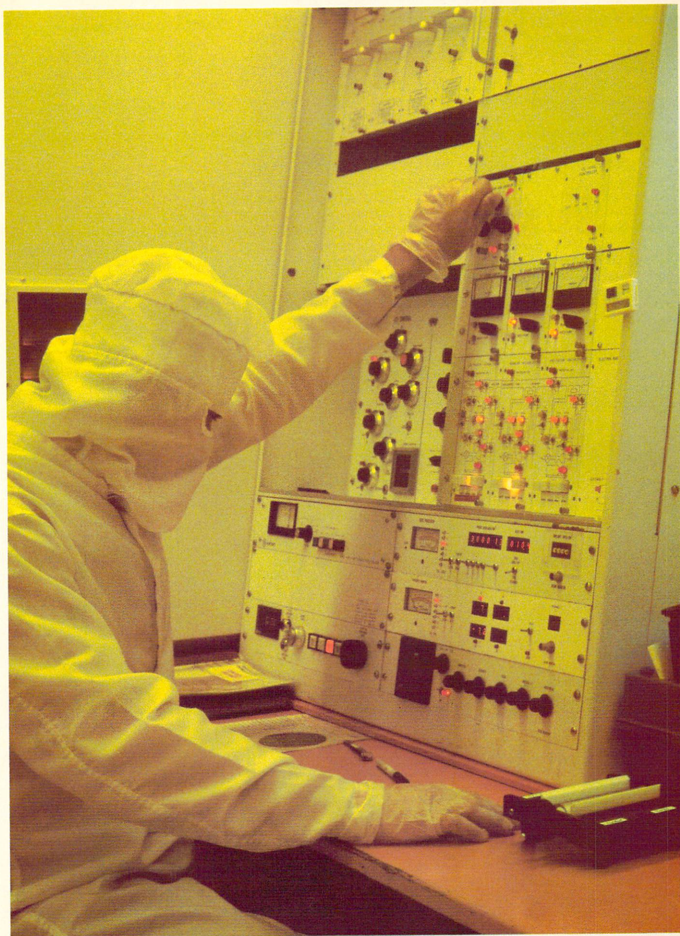
Newer, more complex circuits are sometimes "doped" using extremely accurate ion implantation. This is the implanter control panel.
