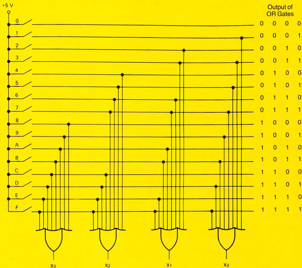
Figure 11. Hex-to-Binary Encoder
