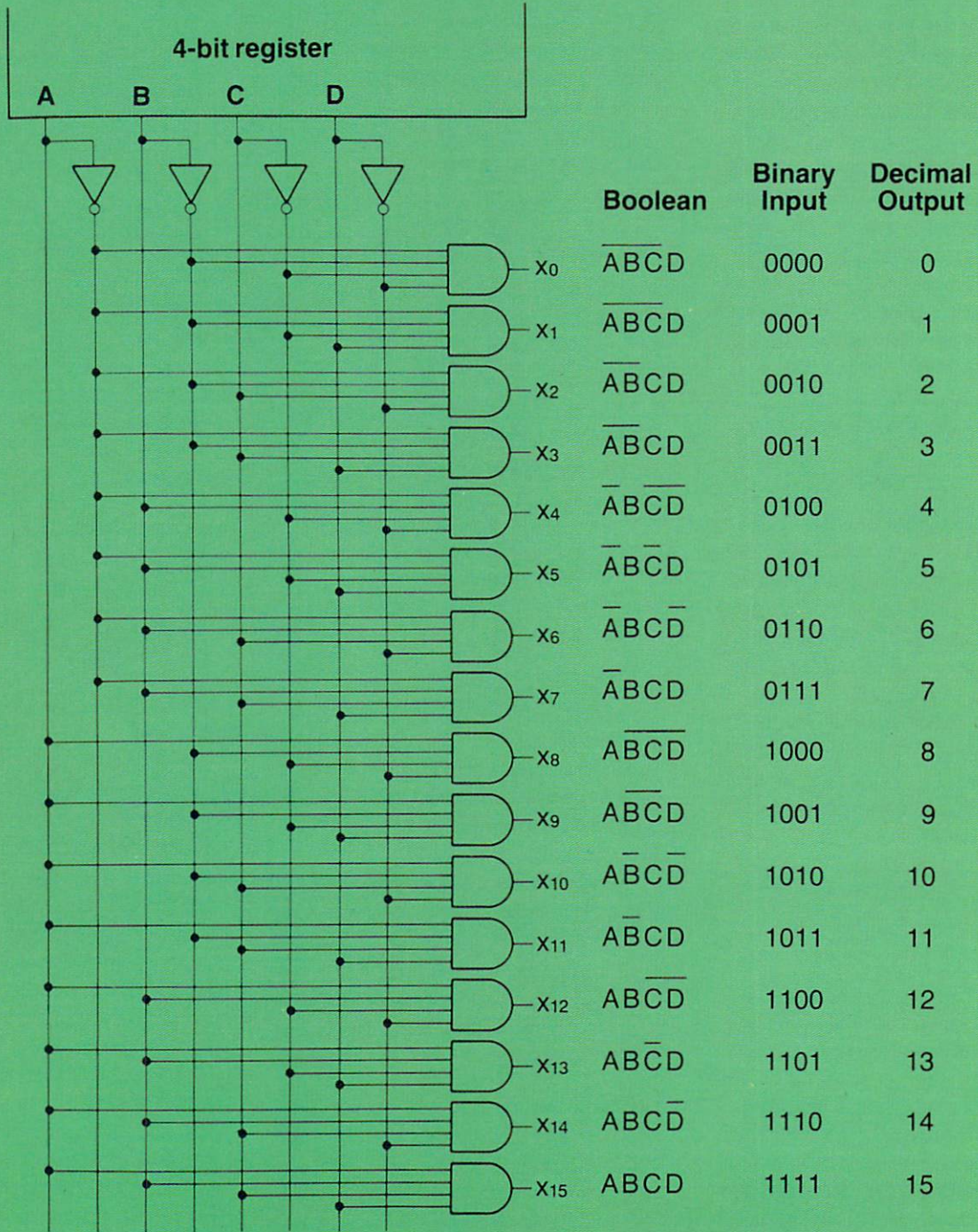
Figure 10. Binary-to-Decimal Decoder
