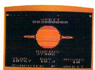
VISIBLE SOLAR SYSTEM
