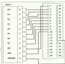
36 WAY AMPHENOL PLUG WIRING SIDE (PINS 14-32 ALL GND).
