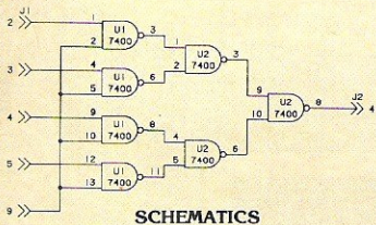
SCHEMATICS
