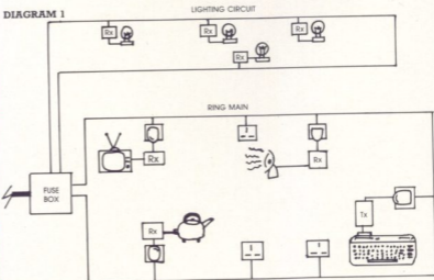
(Tx = Transmitter, Rx = Receiver)
