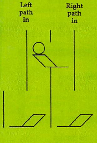
Figure 2. Loaded Trigger
