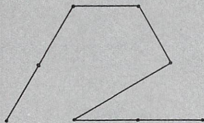
Figure 2: Generator, Program 3
