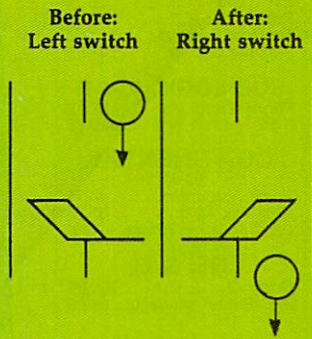
Figure 1. Trigger States
