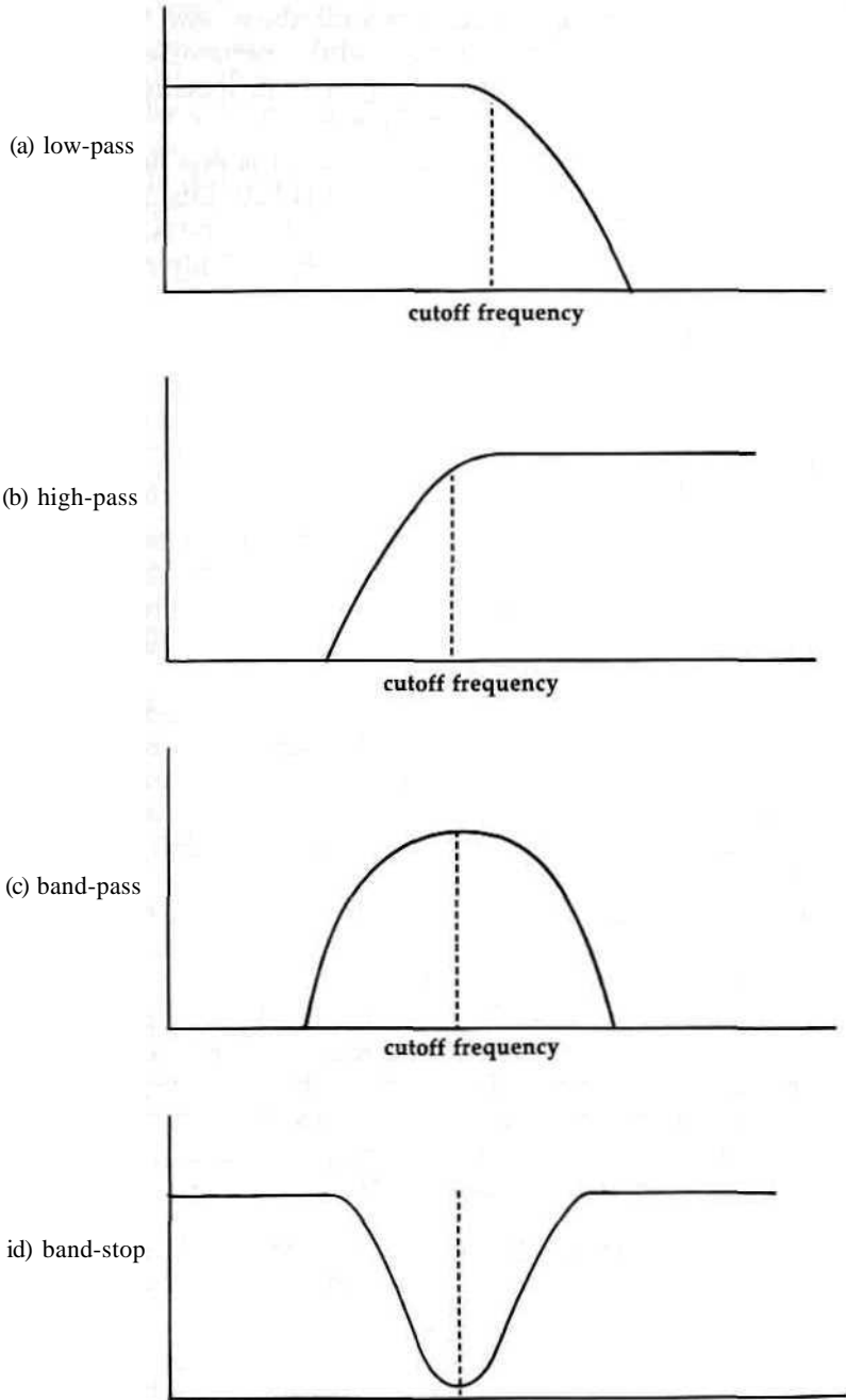
Figure 8-14. Filter Types
