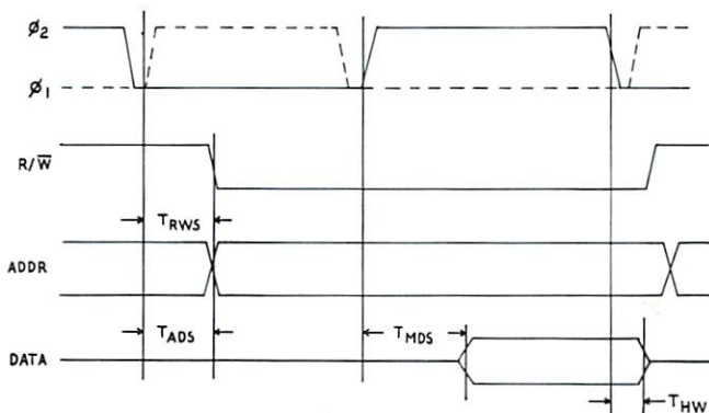
Figure 1. 6502 Write Timing
